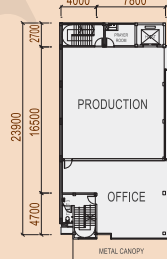
1ST FLOOR
