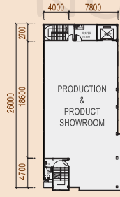
2ND FLOOR
